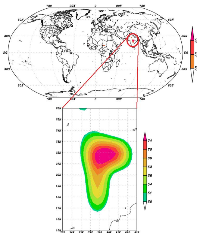
Figure 6. The most intense TU50c recorded in June (June 4, 1992) in the period 1948-2020
